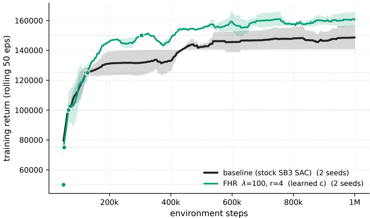
HumanoidStandup-v5 - \lambda 100 -r4 vs baseline (training stream)
