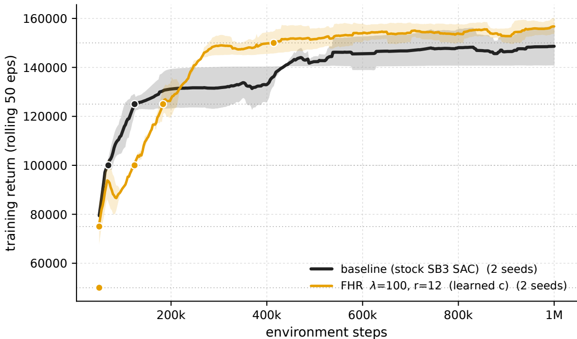
HumanoidStandup-v5 - \lambda 100 \cdot r 12 vs baseline (training stream)
