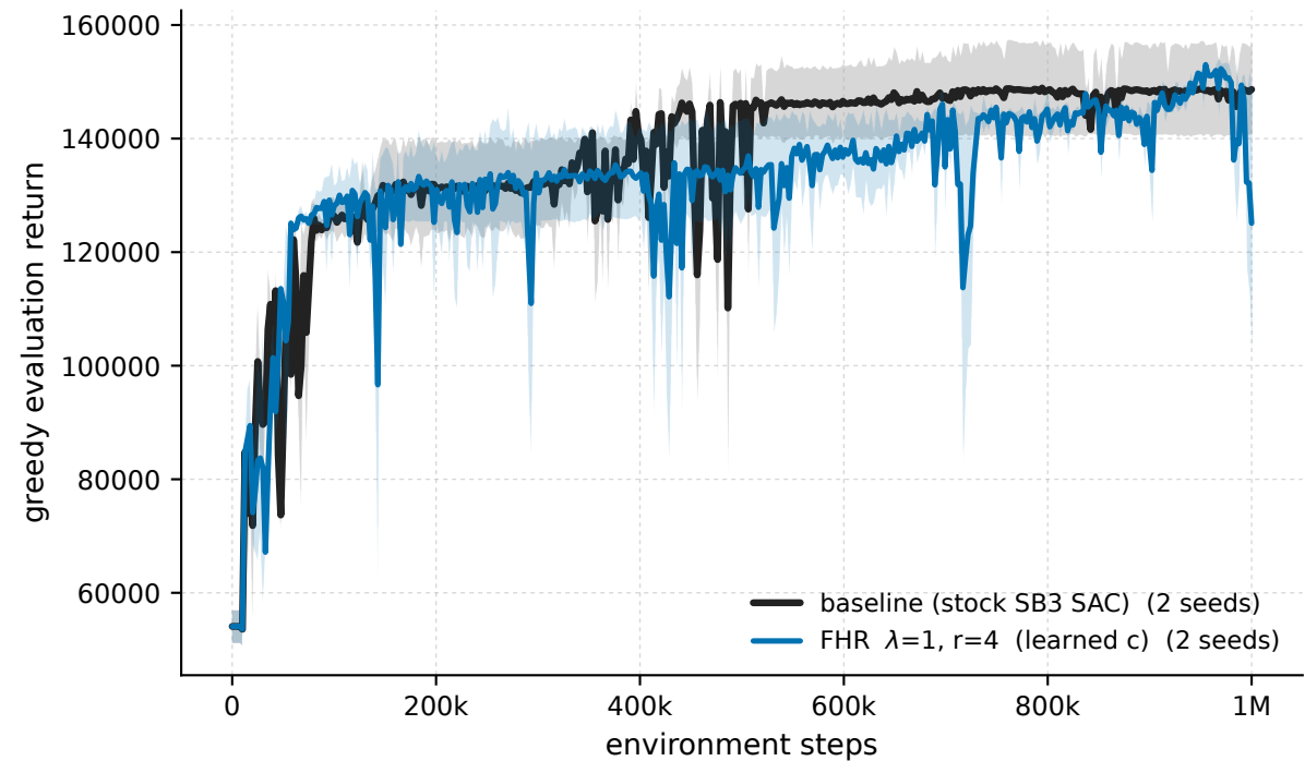
HumanoidStandup-v5 - \lambda 1 \cdot r4 vs baseline (greedy eval)
