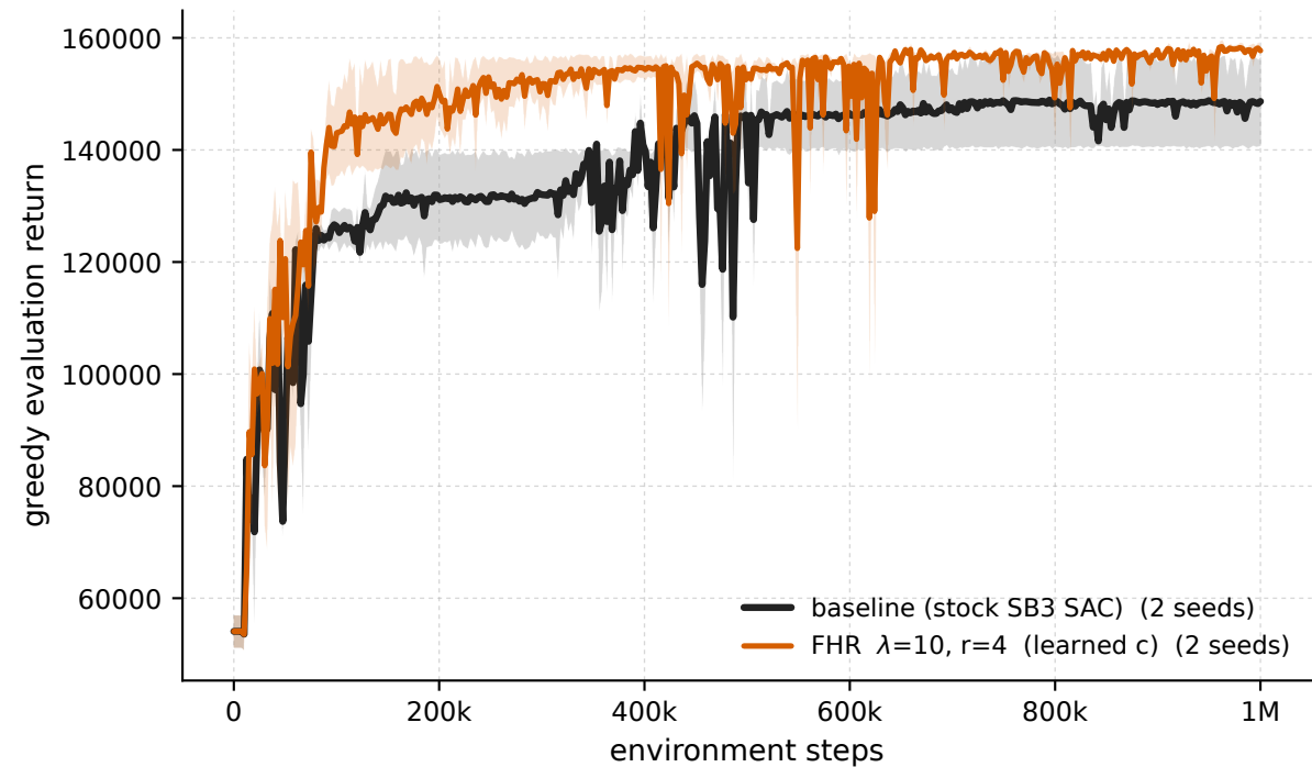
HumanoidStandup-v5 - \lambda 10 \cdot r4 vs baseline (greedy eval)
