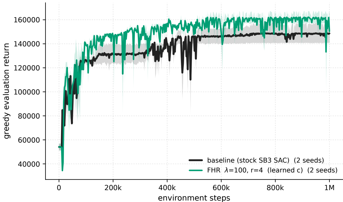
HumanoidStandup-v5 - \lambda 100 \cdot r4 vs baseline (greedy eval)
