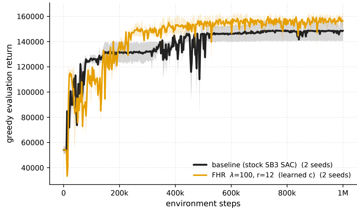
HumanoidStandup-v5 - \lambda 100 \cdot r 12 vs baseline (greedy eval)
