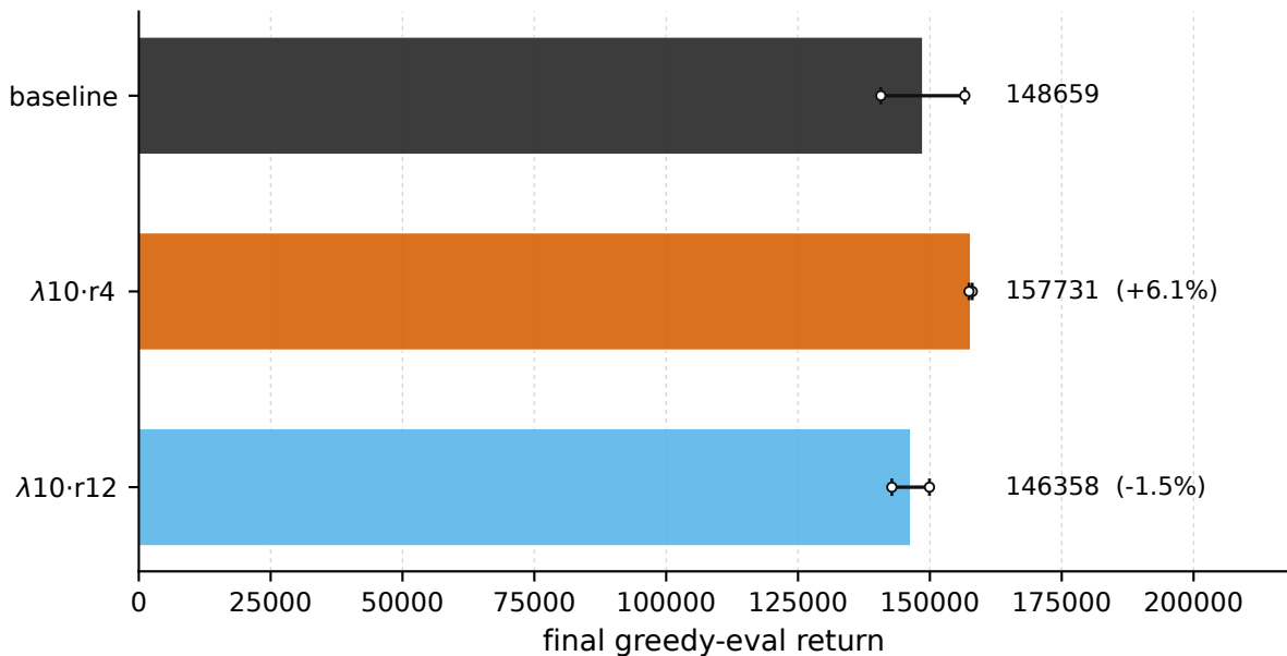
HumanoidStandup-v5 - final return, \lambda = 10 vs baseline
