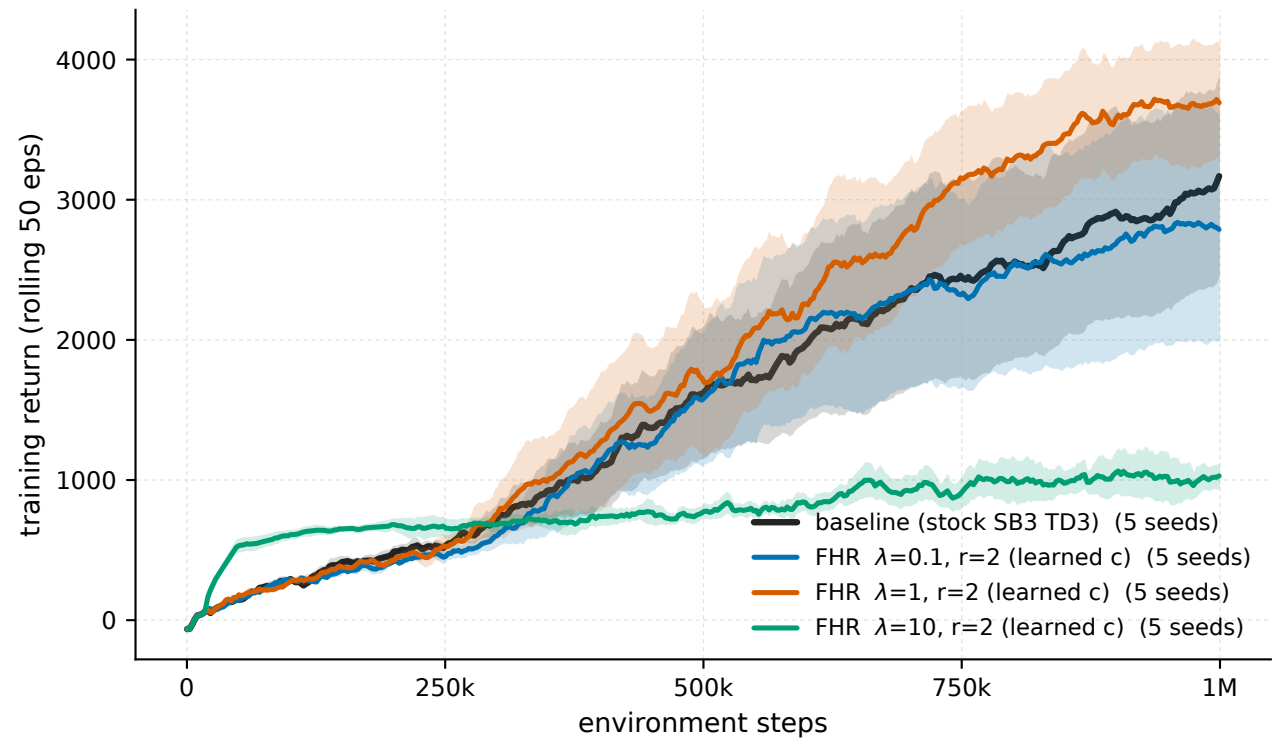
Ant-v5 - all arms (train)
