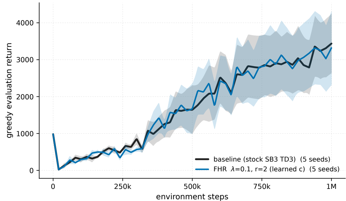
Ant-v5 - \lambda 0.1 \cdot r_2 vs baseline (greedy eval)
