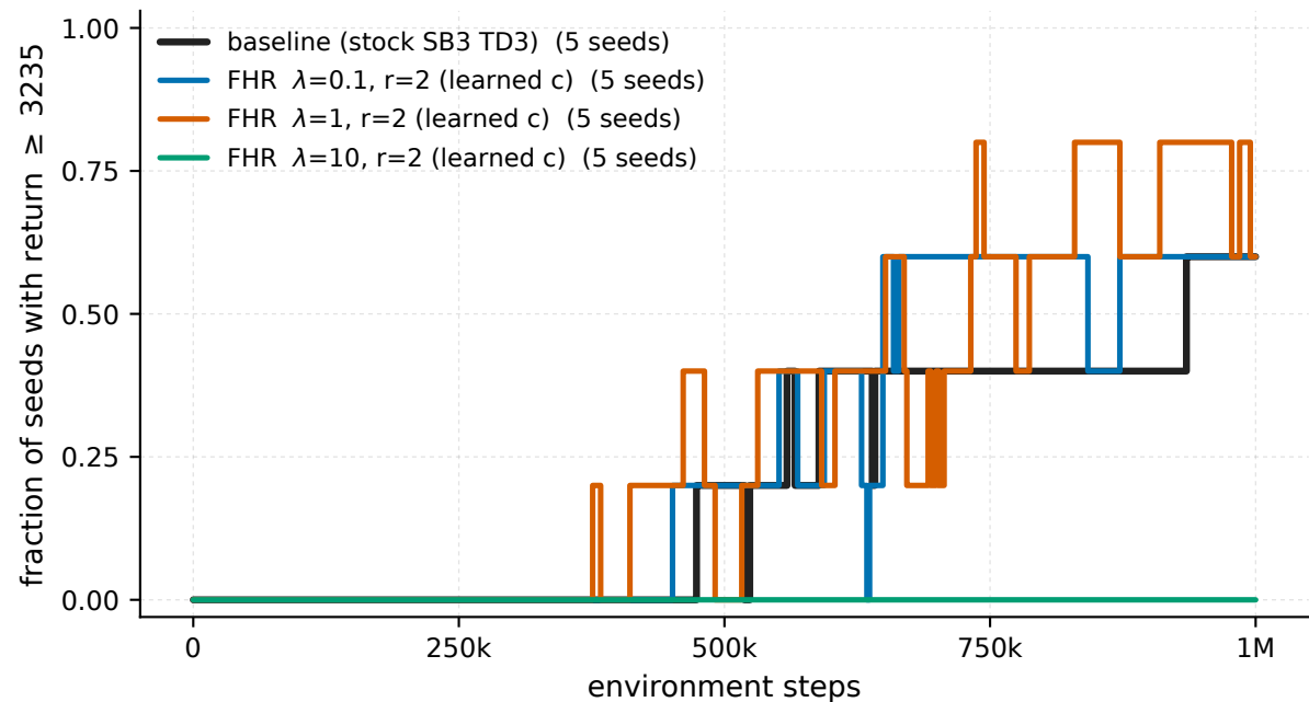
Ant-v5 - seeds above 3235 (eval)
