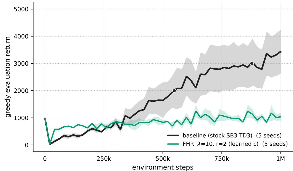
Ant-v5 - \lambda 10 \cdot r_2 vs baseline (greedy eval)
