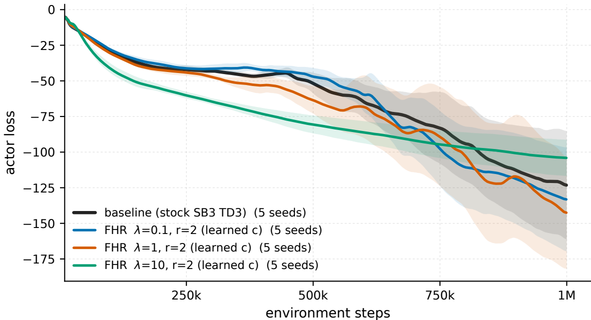
Ant-v5 - actor loss
