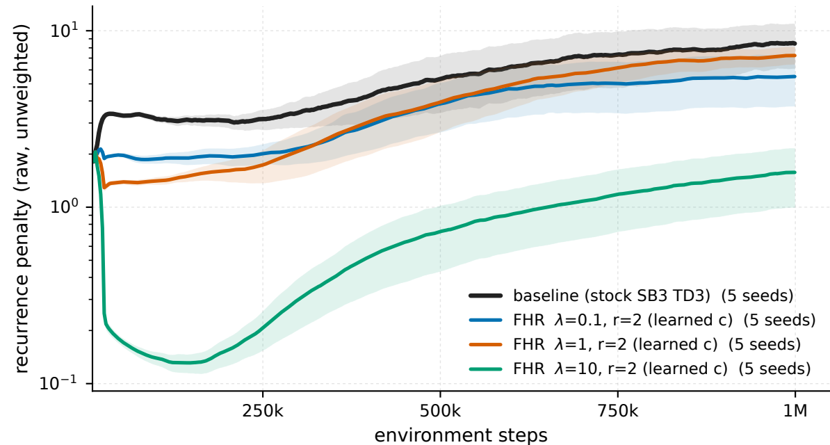
Ant-v5 - recurrence penalty (raw, unweighted)
