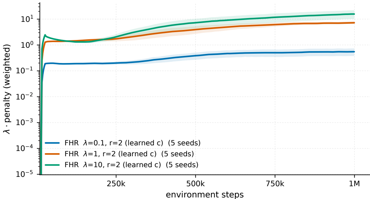
Ant-v5 - \lambda \cdot \text{penalty} (weighted)
