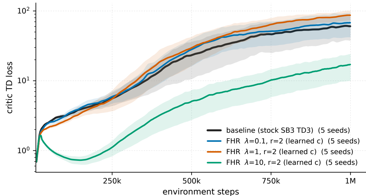
Ant-v5 - critic TD loss
