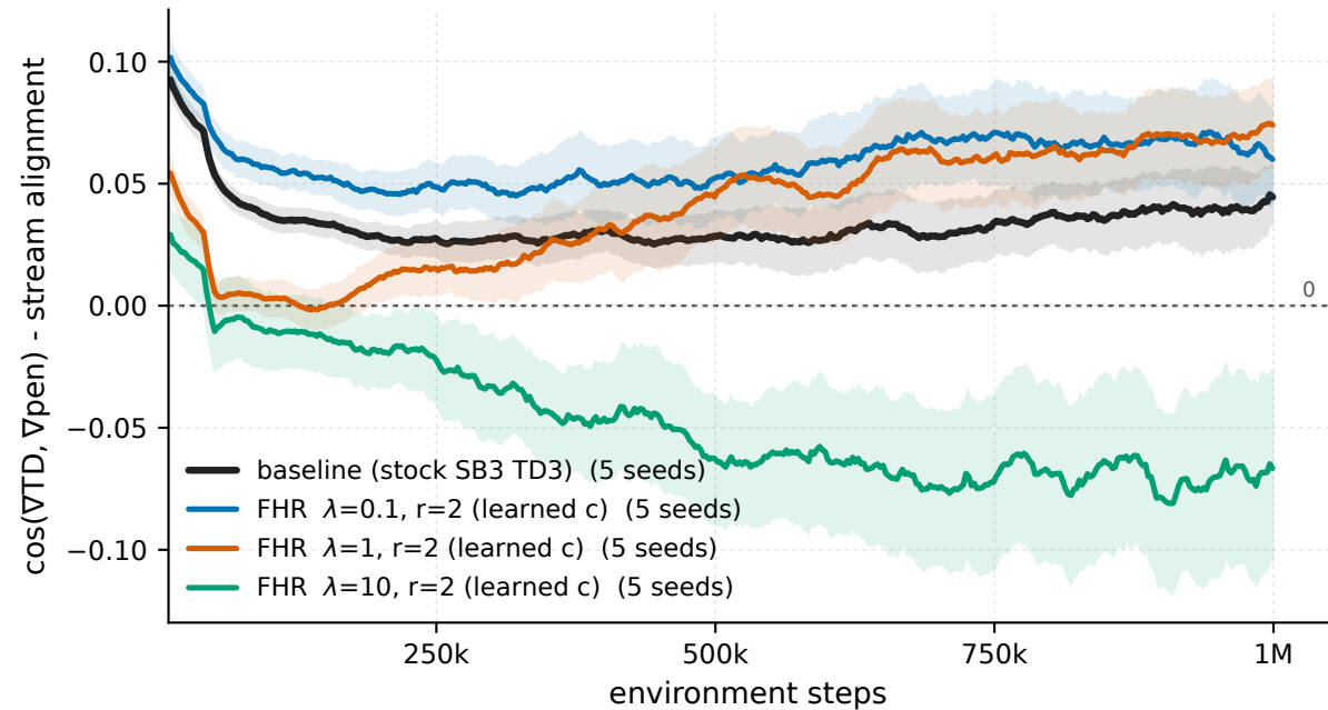
Ant-v5 - \cos(\nabla_{TD}, \nabla_{pen}) - stream alignment
