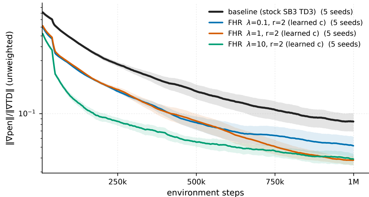
Ant-v5 - \|\nabla \text{pen}\|/\|\nabla \text{TD}\| (unweighted)
