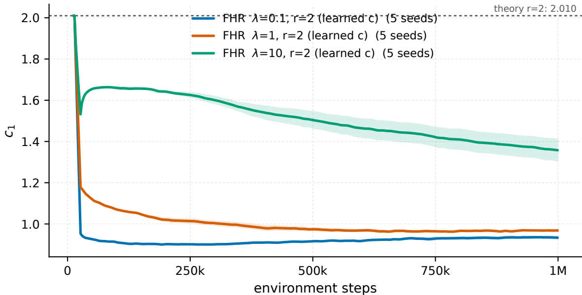
Ant-v5 - recurrence coefficient c_1 vs the Bellman theory value
