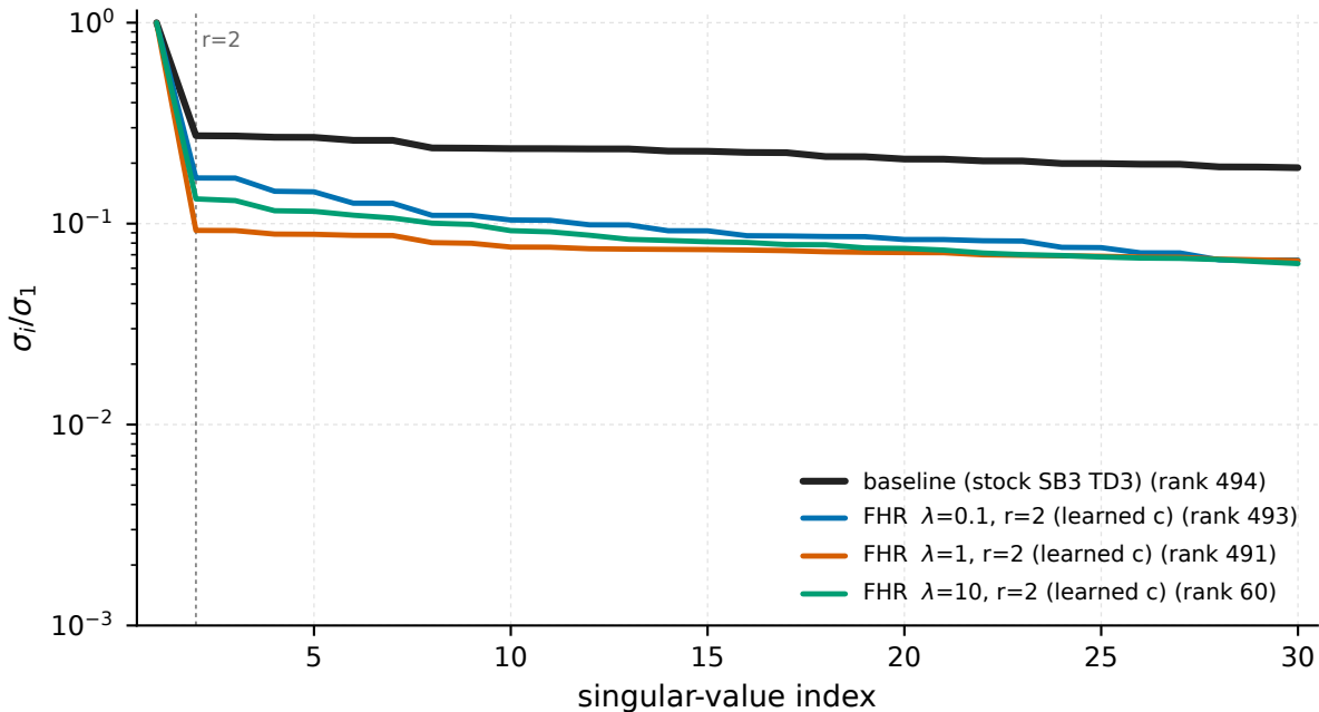
Ant-v5 - Hankel( \pi(s_t)_2 ) of the final policy (action dim 2)
