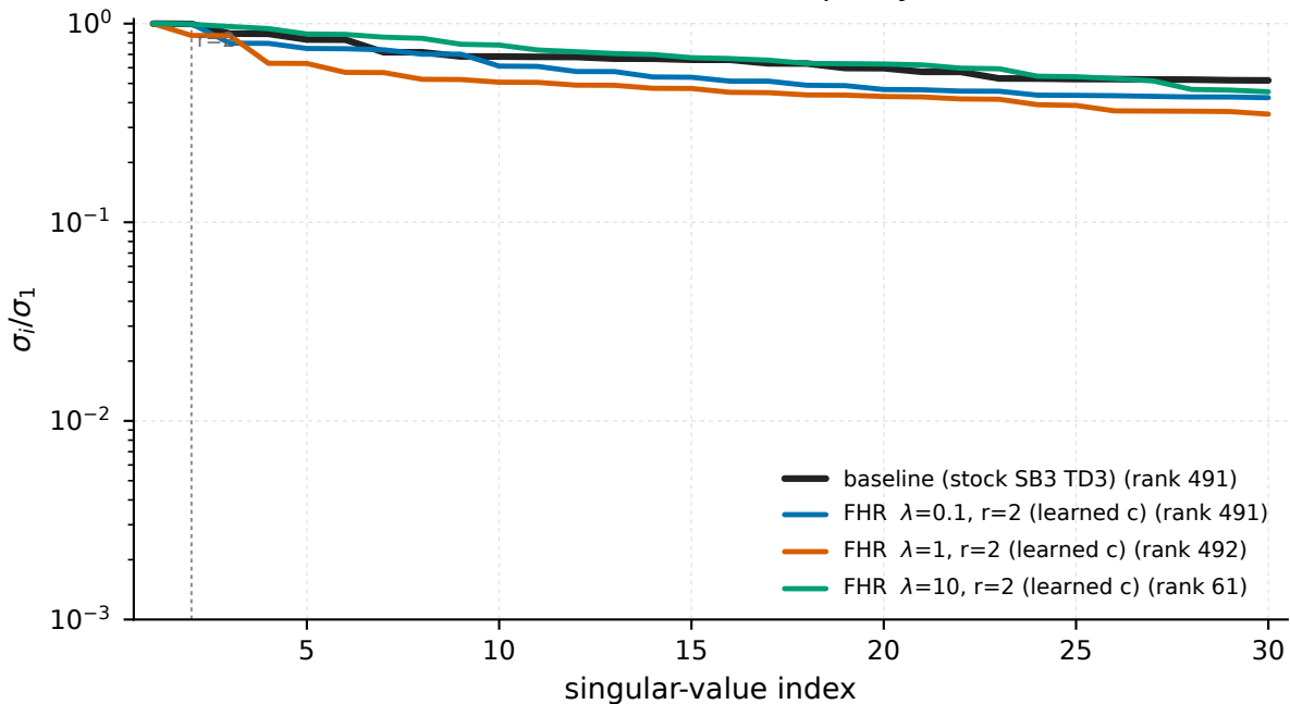
Ant-v5 - \text{Hankel}(\pi(s_t)_4) of the final policy (action dim 4)
