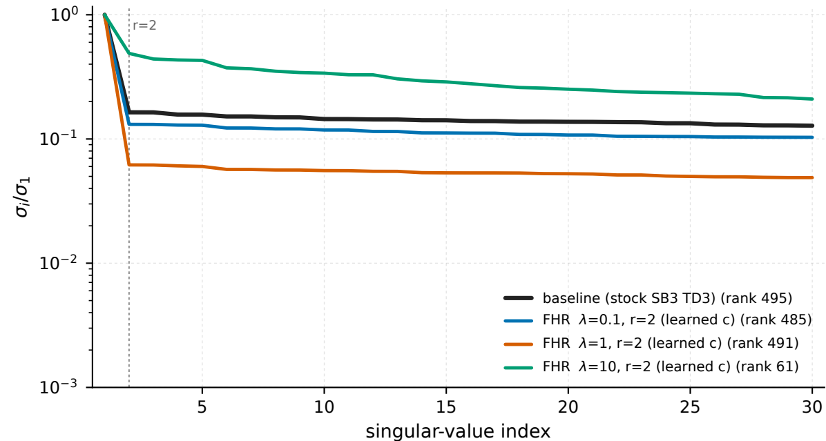
Ant-v5 - Hankel( \pi(s_t)_5 ) of the final policy (action dim 5)
