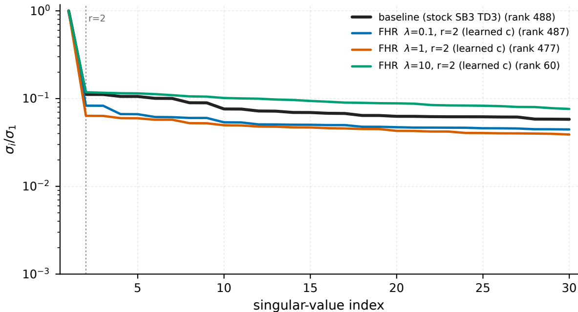
Ant-v5 - Hankel( \pi(s_t)_7 ) of the final policy (action dim 7)
