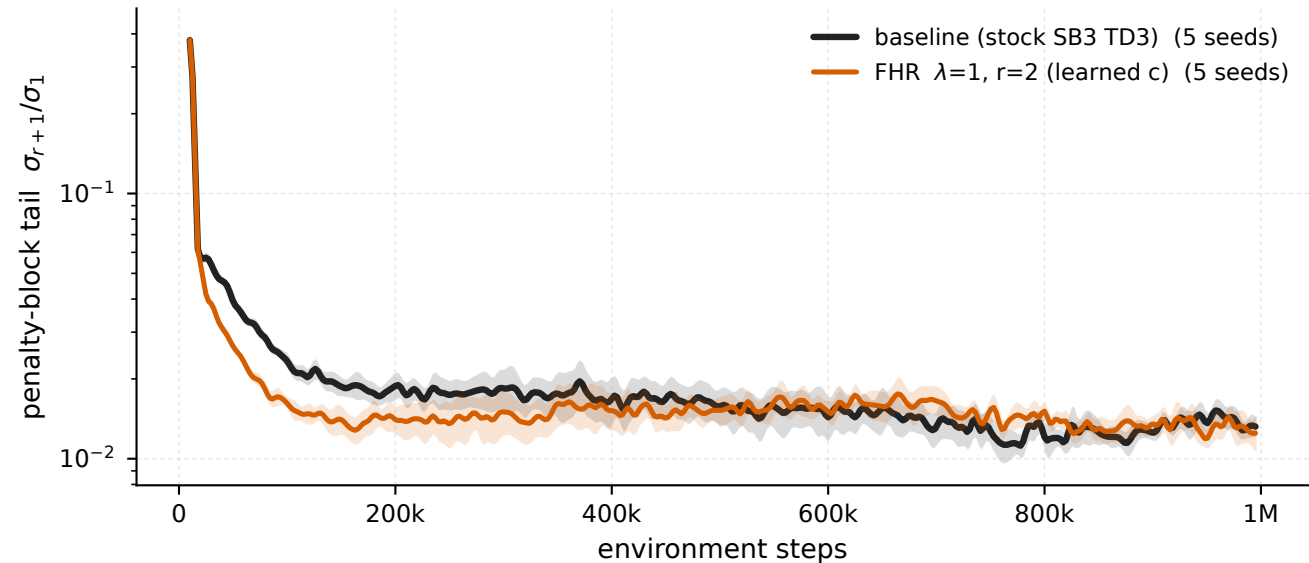
Ant-v5 - \lambda 1 \cdot r_2 vs baseline, penalised windows penalty-block tail \sigma_{r+1}/\sigma_1
