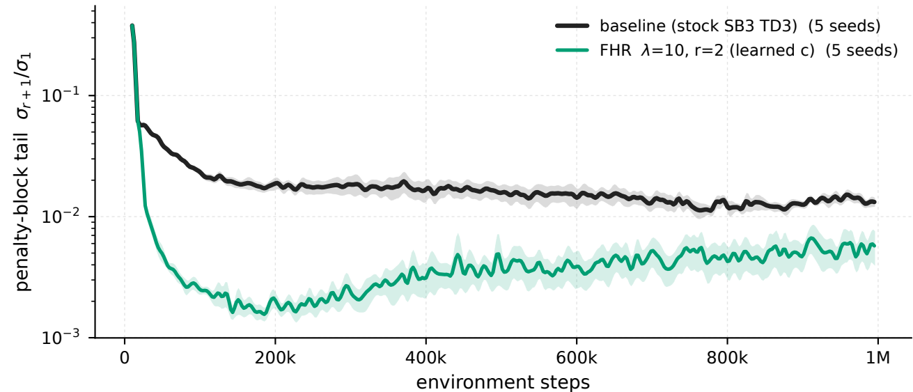
Ant-v5 - \lambda 10 \cdot r_2 vs baseline, penalised windows penalty-block tail \sigma_{r+1}/\sigma_1
