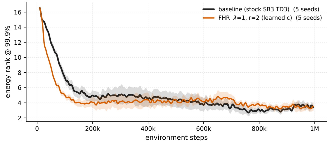
Ant-v5 - \lambda 1 \cdot r 2 vs baseline, penalised windows energy rank @ 99.9%
