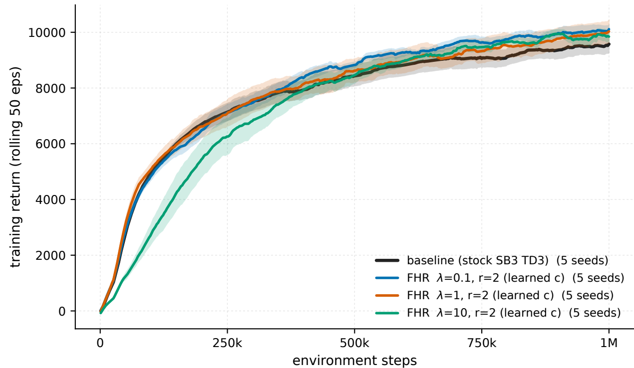
HalfCheetah-v5 - all arms (train)
