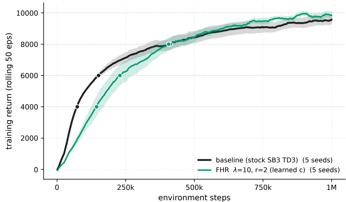
HalfCheetah-v5 - \lambda 10 \cdot r_2 vs baseline (training stream)
