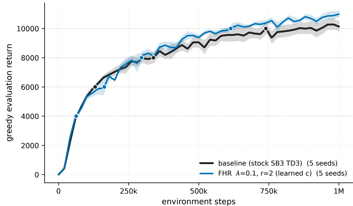
HalfCheetah-v5 - \lambda 0.1 \cdot r_2 vs baseline (greedy eval)
