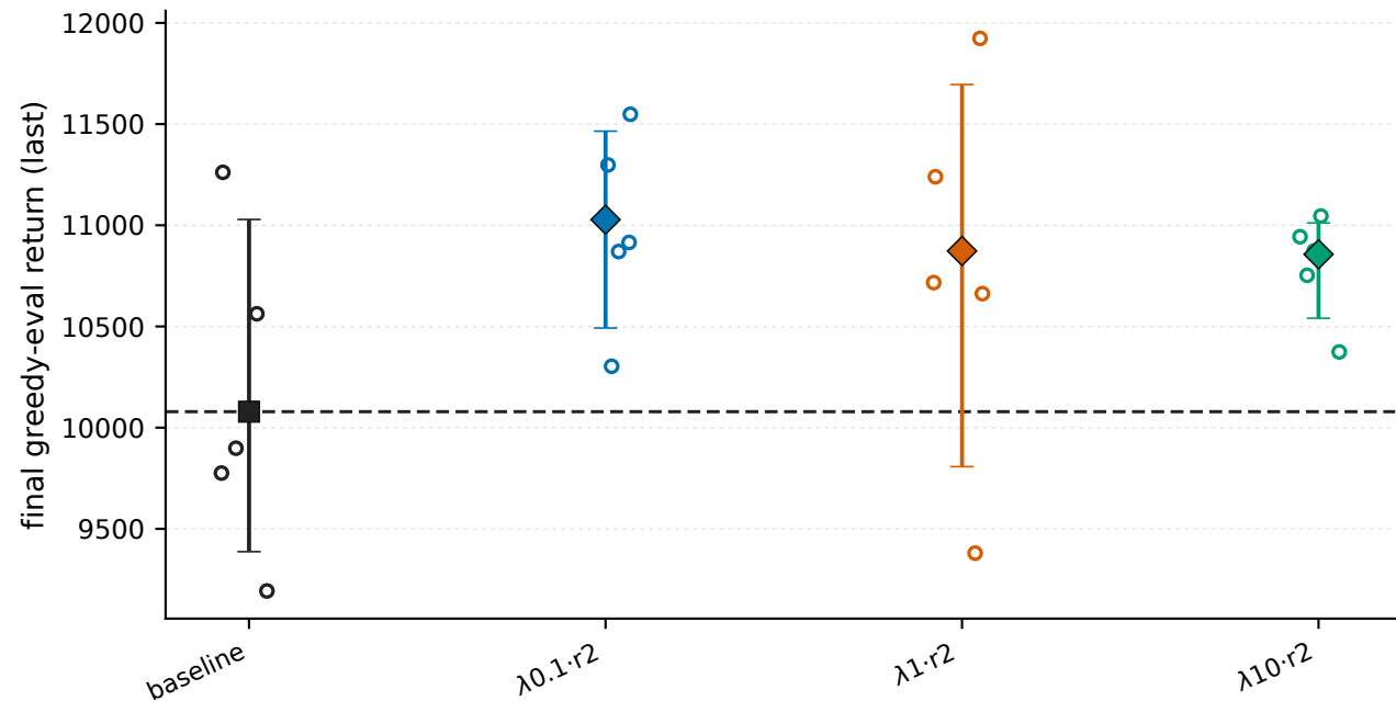
HalfCheetah-v5 - final return per arm: seeds (o), IQM with 95% bootstrap CI; dashed = baseline IQM
