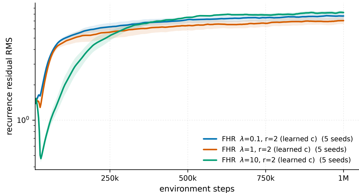
HalfCheetah-v5 - recurrence residual RMS
