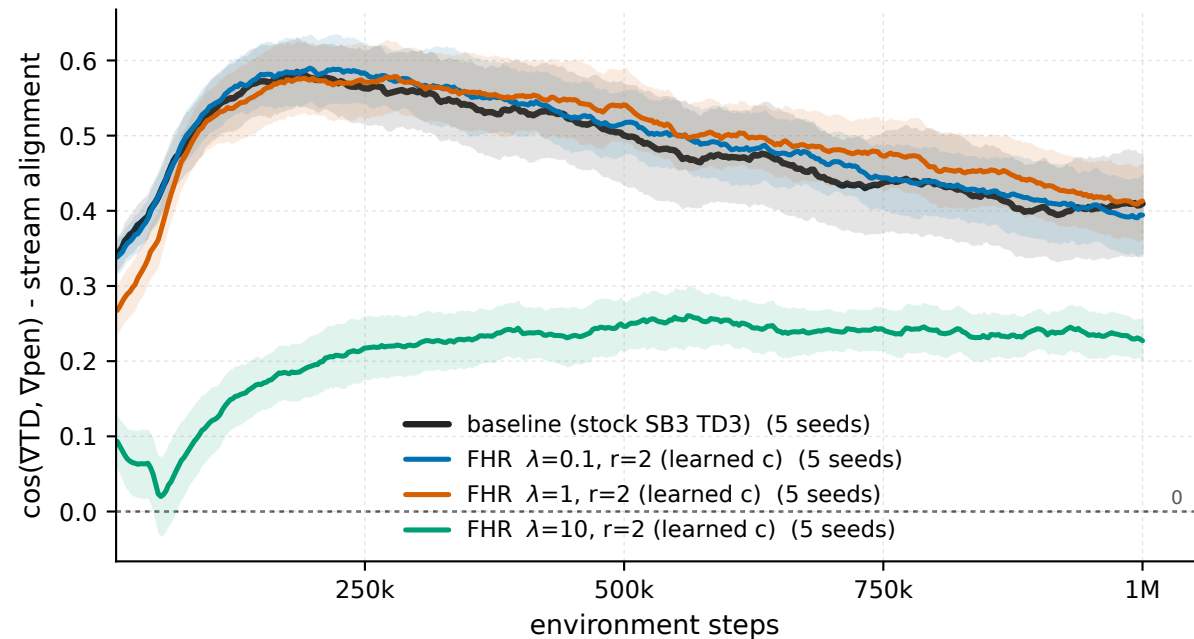
HalfCheetah-v5 - \cos(\nabla_{TD}, \nabla_{pen}) - stream alignment
