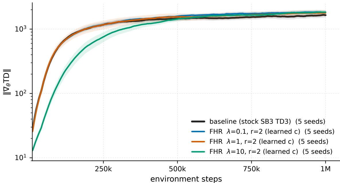
HalfCheetah-v5 - \|\nabla_{\theta}TD\|
