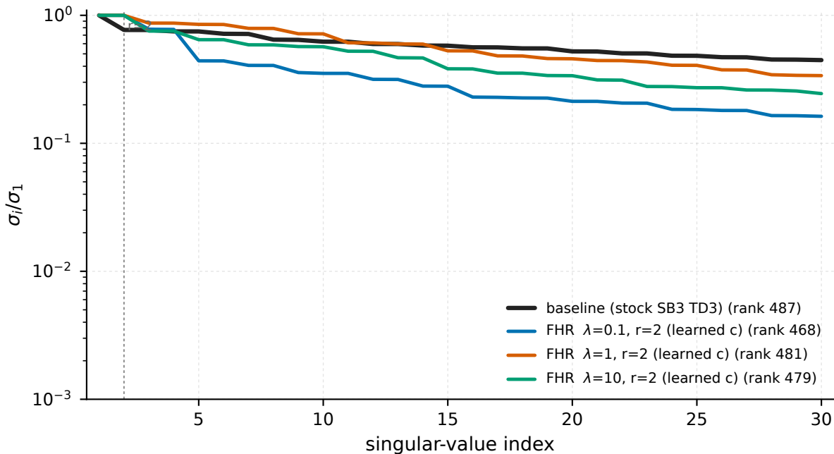
HalfCheetah-v5 - \text{Hankel}(\pi(s_t)_4) of the final policy (action dim 4)
