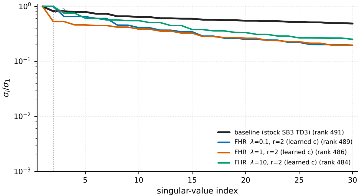
HalfCheetah-v5 - Hankel( \pi(s_t)_5 ) of the final policy (action dim 5)
