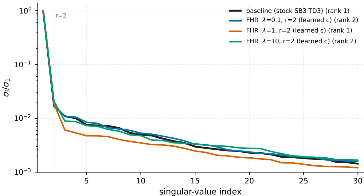
HalfCheetah-v5 - Hankel( Q(s_t, \pi(s_t)) ) of the final policy (critic trace)
