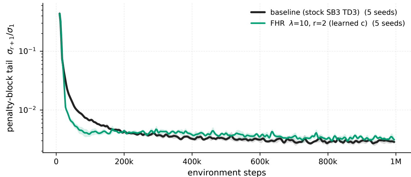
HalfCheetah-v5 - \lambda 10 \cdot r_2 vs baseline, penalised windows penalty-block tail \sigma_{r+1}/\sigma_1
