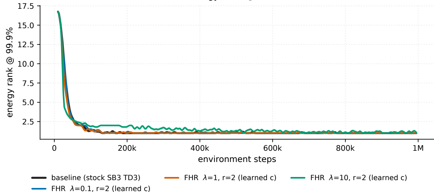
HalfCheetah-v5 - penalised windows, all arms energy rank @ 99.9%
