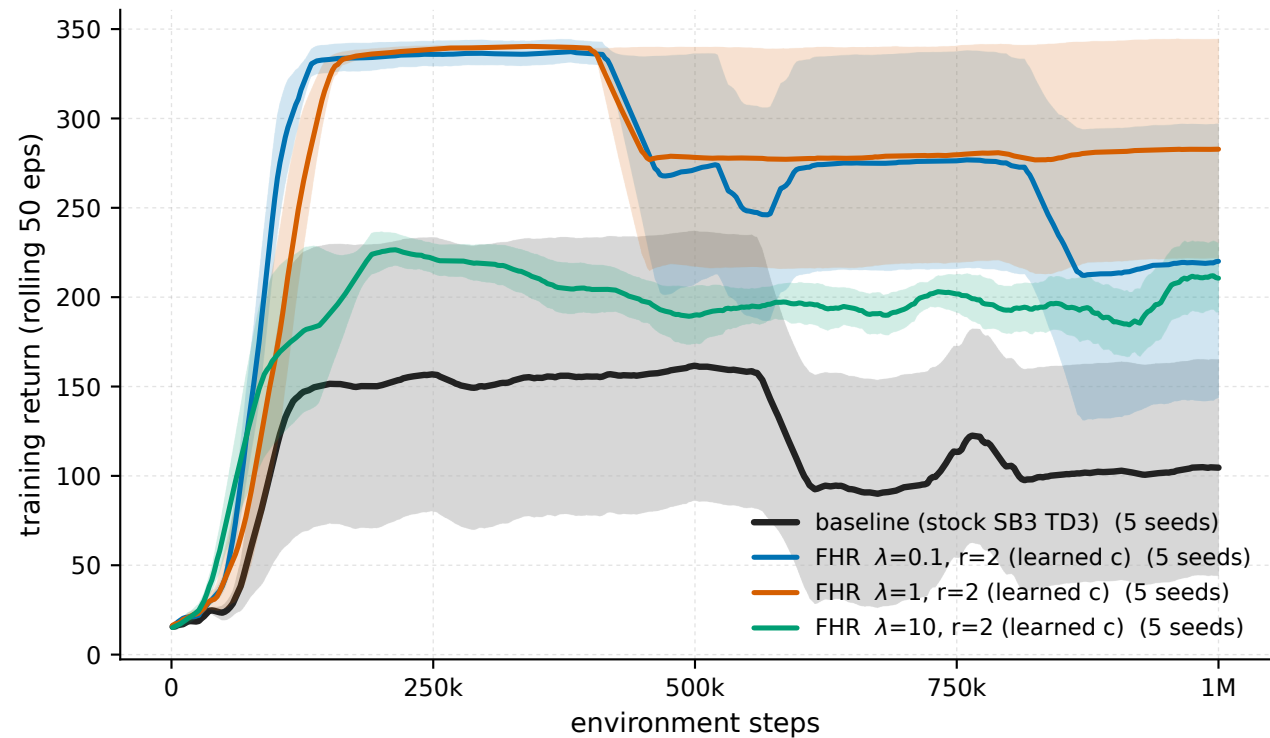
Swimmer-v5 - all arms (train)
