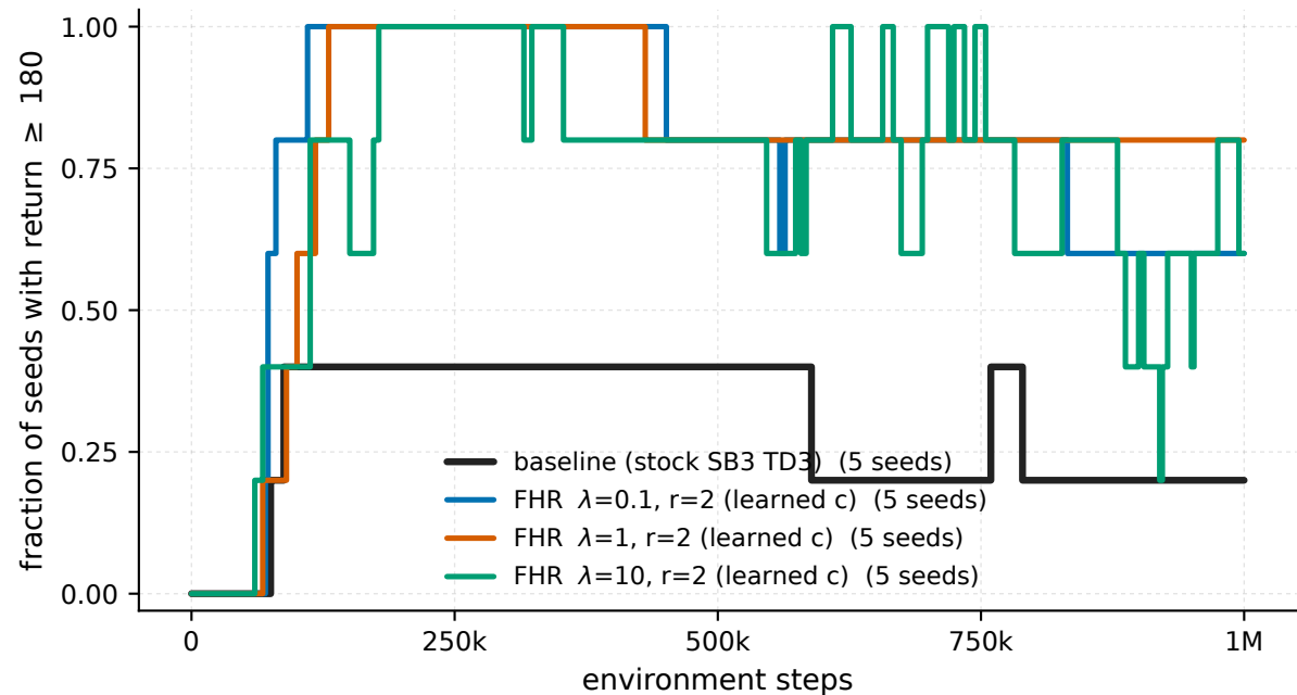
Swimmer-v5 - seeds above 180 (eval)
