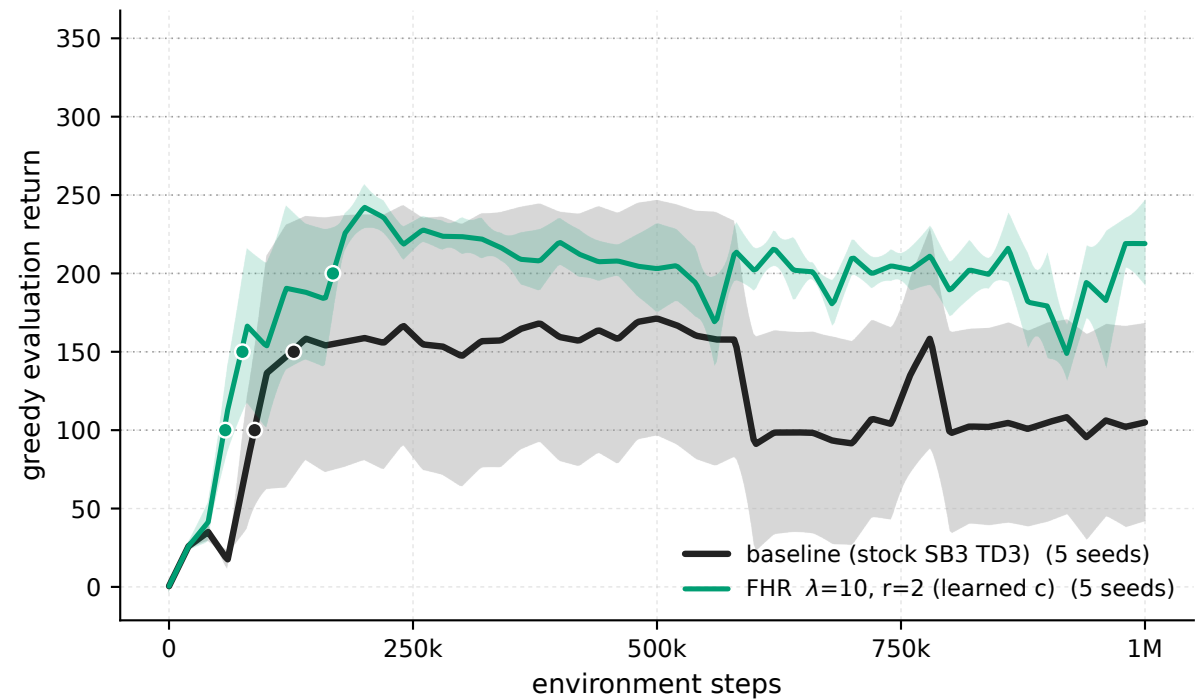
Swimmer-v5 - \lambda 10 \cdot r2 vs baseline (greedy eval)
