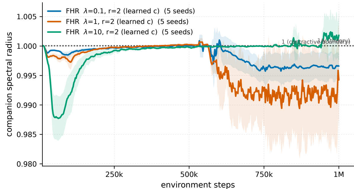
Swimmer-v5 - companion spectral radius
