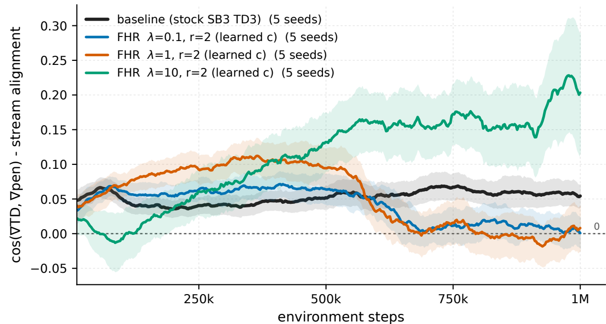
Swimmer-v5 - \cos(\nabla_{TD}, \nabla_{pen}) - stream alignment
