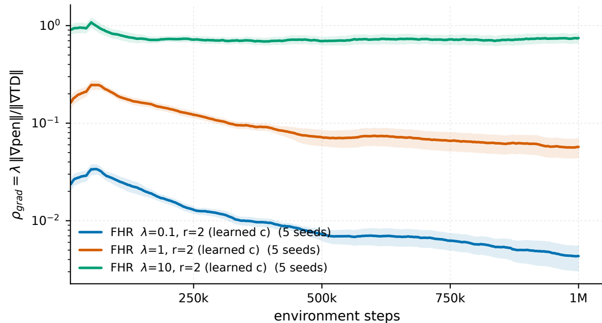
Swimmer-v5 - \rho_{grad} = \lambda \|\nabla pen\|/\|\nabla TD\|
