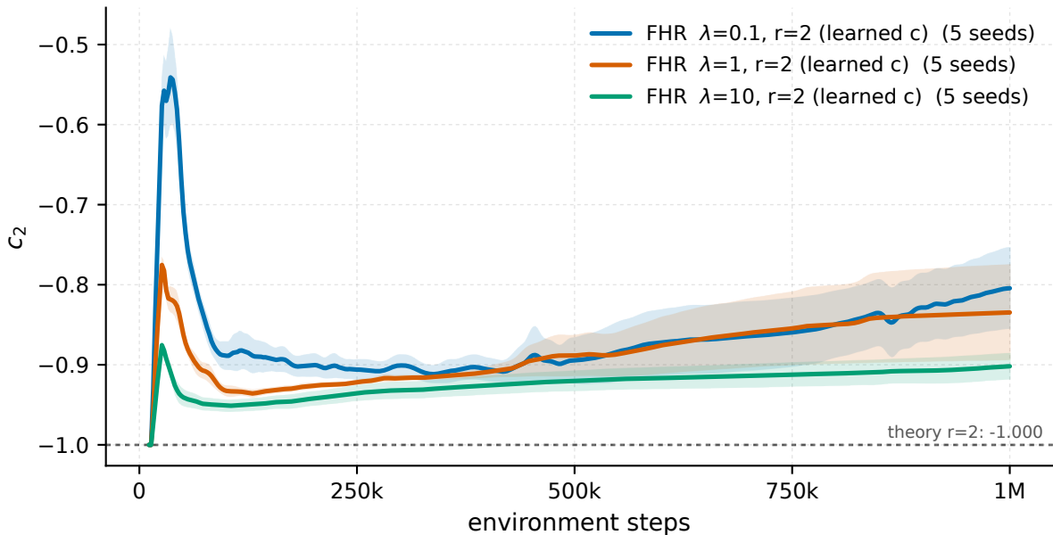
Swimmer-v5 - recurrence coefficient c_2 vs the Bellman theory value
