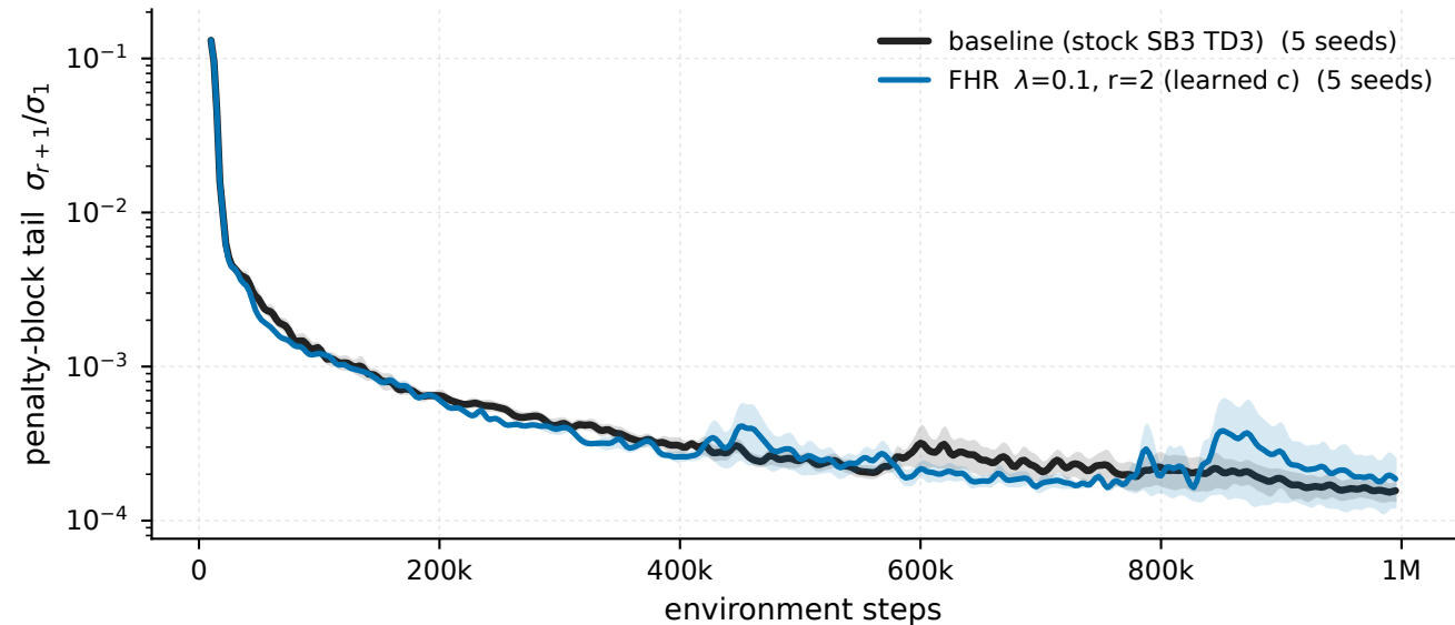
Swimmer-v5 - \lambda 0.1 \cdot r_2 vs baseline, penalised windows penalty-block tail \sigma_{r+1}/\sigma_1
