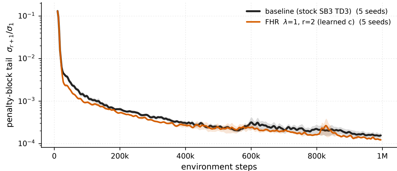
Swimmer-v5 - \lambda 1 \cdot r_2 vs baseline, penalised windows penalty-block tail \sigma_{r+1}/\sigma_1
