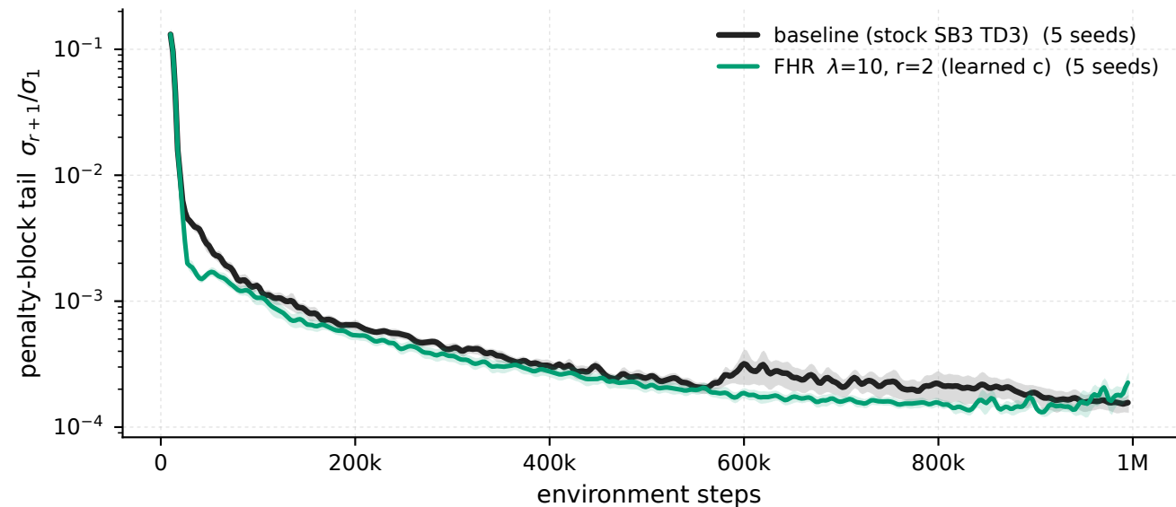
Swimmer-v5 - \lambda 10 \cdot r_2 vs baseline, penalised windows penalty-block tail \sigma_{r+1}/\sigma_1
