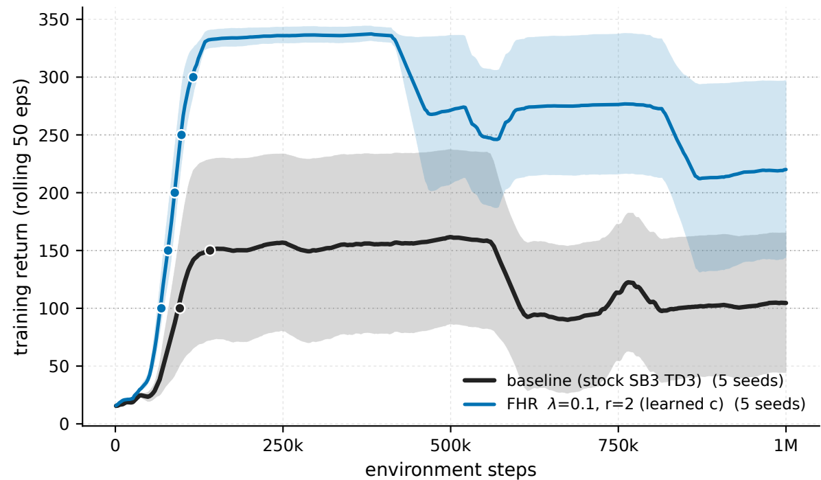
Swimmer-v5 - \lambda 0.1 \cdot r_2 vs baseline (training stream)
