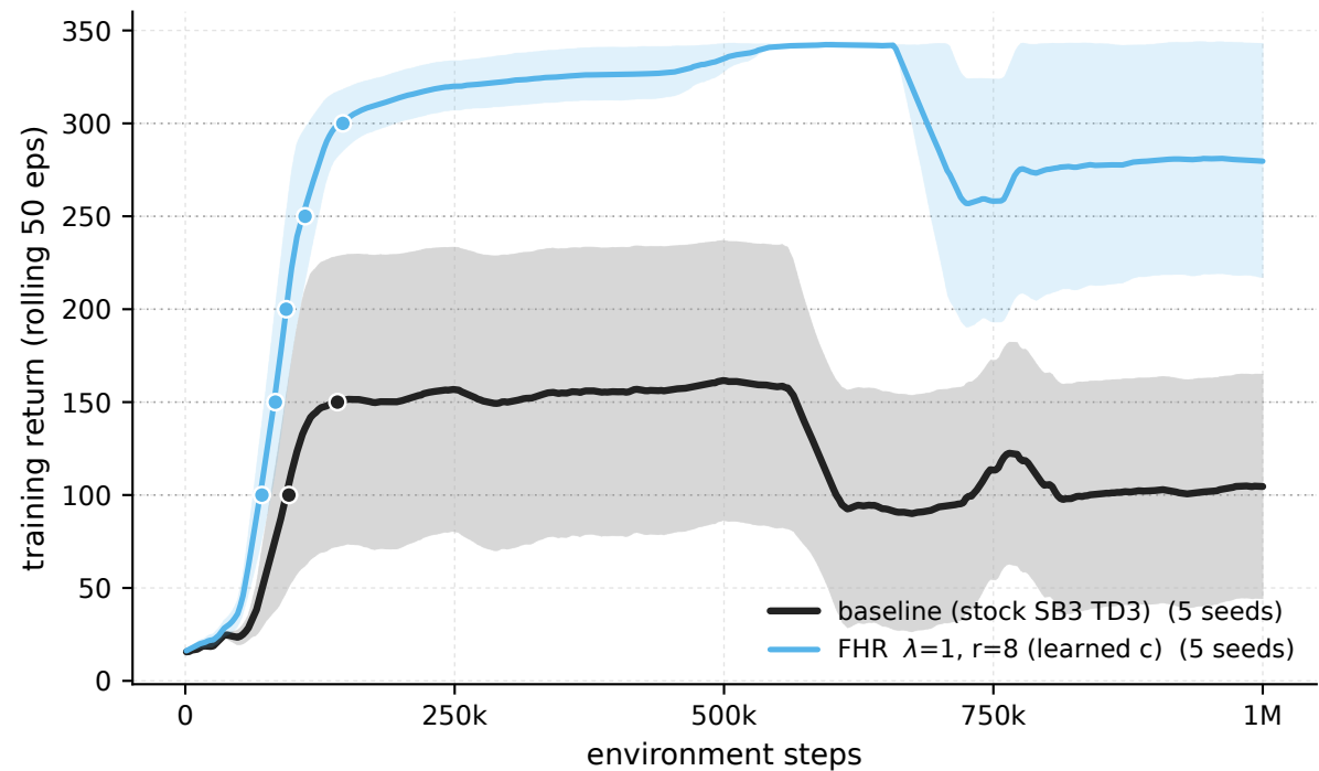
Swimmer-v5 - \lambda 1 \cdot r8 vs baseline (training stream)
