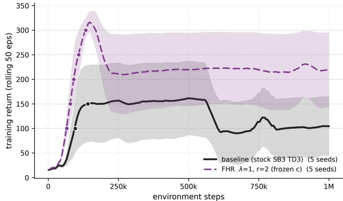
Swimmer-v5 - \lambda 1 \cdot r2 frozen-c vs baseline (training stream)
